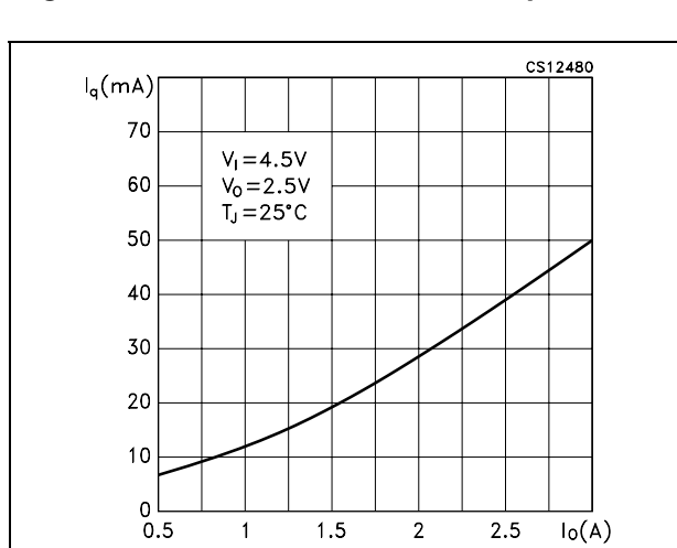
Figure 9. Quiescent current vs output current
